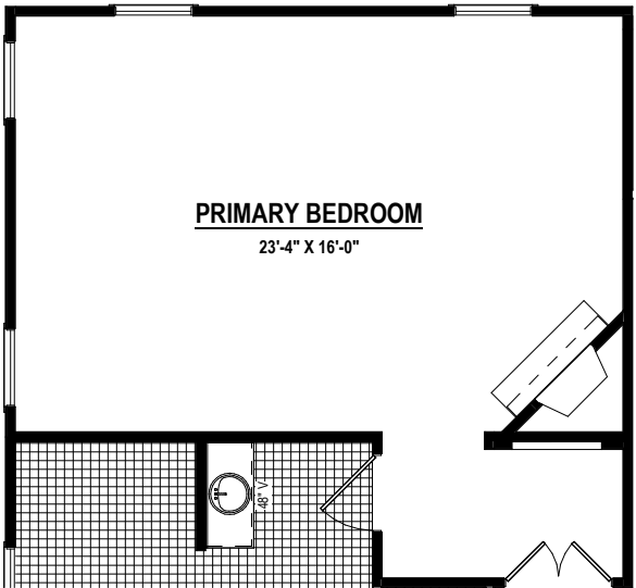
GAS FIREPLACE AT PRIMARY BEDROOM Custom Option
