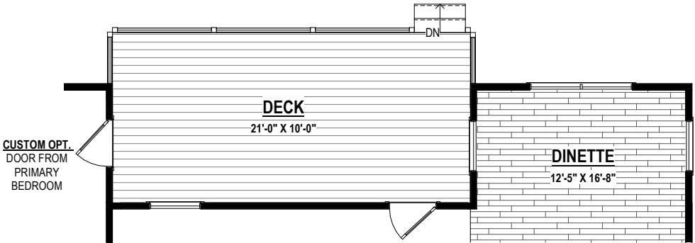
WOOD DECK W/ DINETTE EXTENSION (144 SF ± 84 SF ±) Option #15000 8' Option #15125 9' Option #15126
