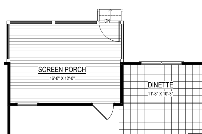
SCREEN PORCH W/ DINETTE (160 SF ± 74 SF ±) Option #15506 Option #15047 Option #15516 Option #15046
