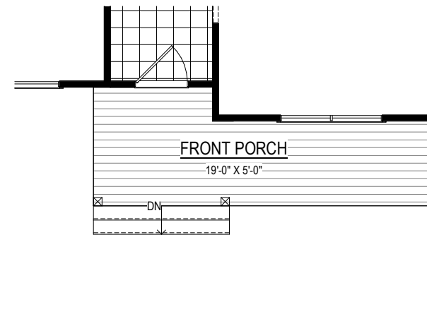
FULL FRONT PORCH (92 SF ±) Wood Option #15245 Masonry Option #15240
