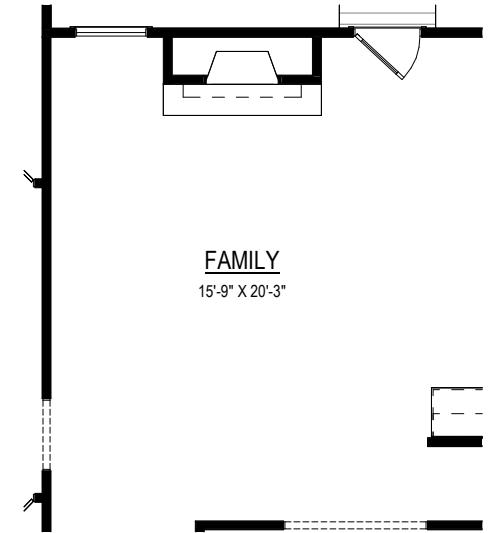
GAS FIREPLACE AT FAMILY ROOM 8'-0" Option #35004 9'-0" Option #35008
