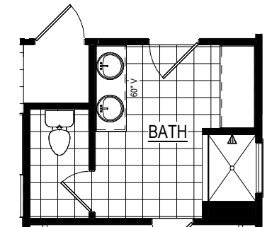
PRIMARY BATH W/ MAKEUP VANITY
