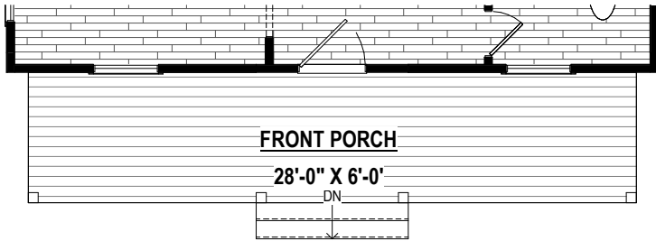
FULL FRONT PORCH (140 SF ±)
