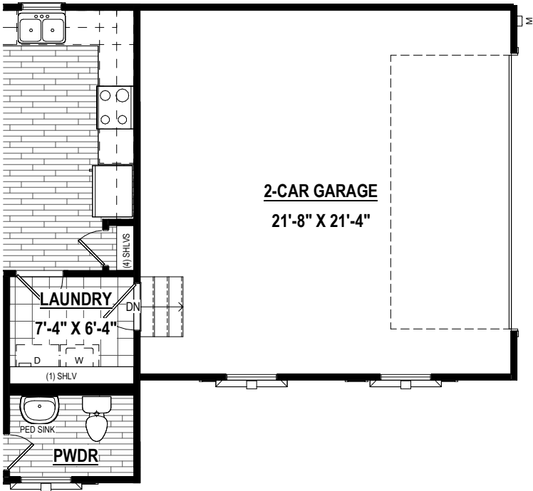
2-CAR SIDE-LOAD GARAGE (484 SF ±) 8'-0" Option #15238 9'-0" Option #15260
