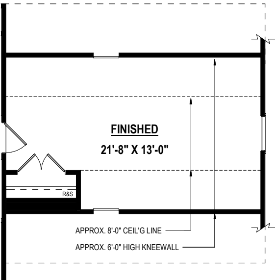
FINISHED ROOM OVER 1-CAR GARAGE (286 S/F ±) Option #15034
