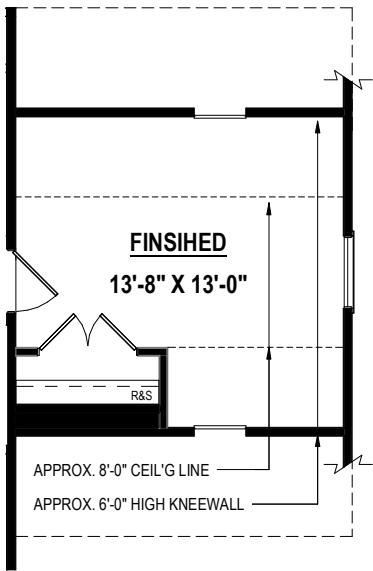
FINISHED ROOM OVER 1-CAR GARAGE (182 S/F ±) Option #15033
