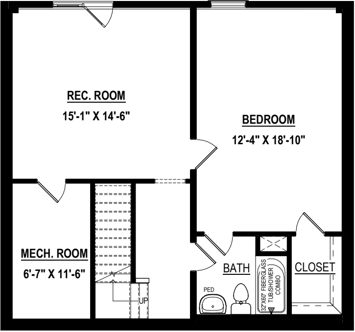
FINISHED BASEMENT W/ (802 S/F ± ) Option #
