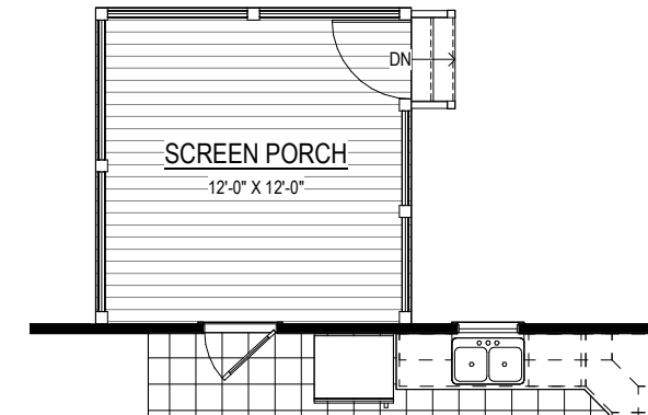
SCREEN PORCH (147 SF ±) Option #15501
