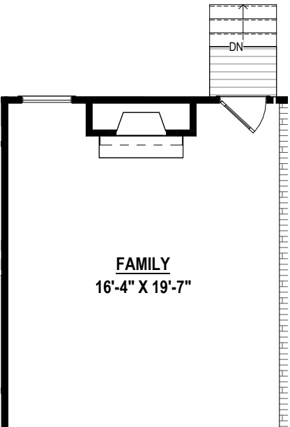
GAS FIREPLACE AT FAMILY ROOM
