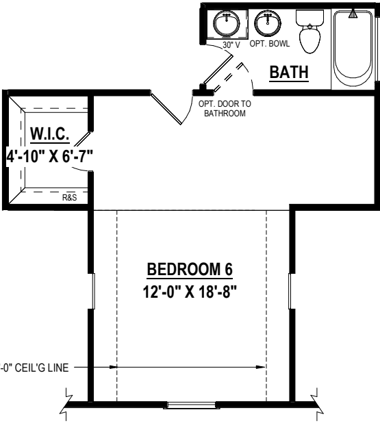
BEDROOM 6 - OVER GARAGE (309 SF ±) Option # 15110
