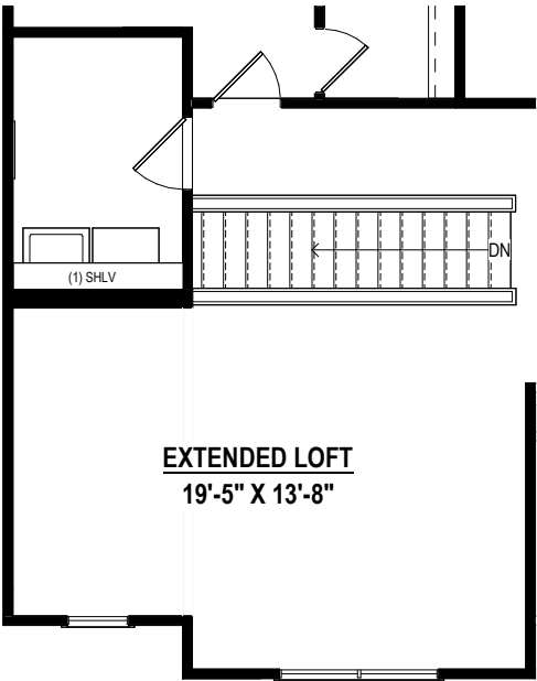
EXTENDED LOFT (77 SF ±) Option # 15186
