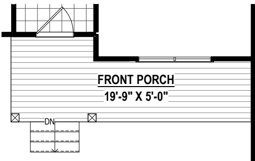
FULL FRONT PORCH (112 SF ±)
