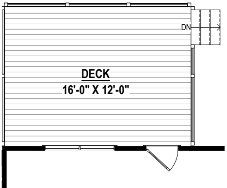
WOOD DECK (189 SF ±)
