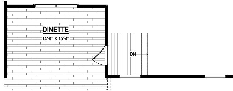
DINETTE EXTENSION (57 SF ±) 8'-0" Option #15125 9'-0" Option #15126
