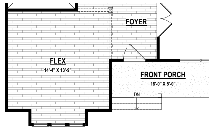
BAY AT FLEX 8'-0" Option #15127 9'-0" Option #15128
