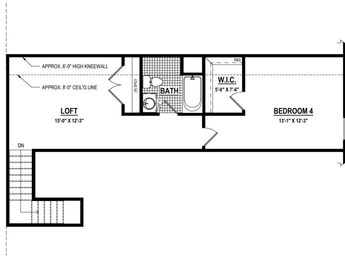
OPTIONAL SECOND FLOOR (581 SF ±) Custom Option
