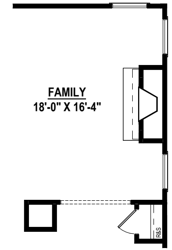
GAS FIREPLACE AT FAMILY ROOM 8'-0" Option #35001 9'-0" Option #35005
