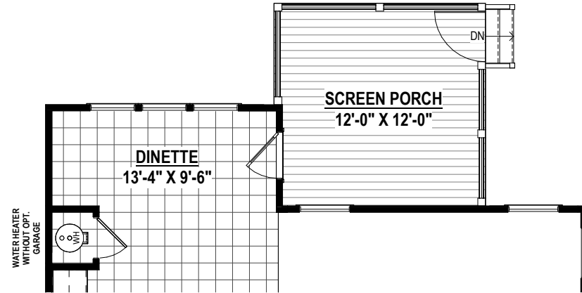
SCREEN PORCH W/ DINETTE (147 SF ± 84 SF ±) Option #15501 Option #15047
