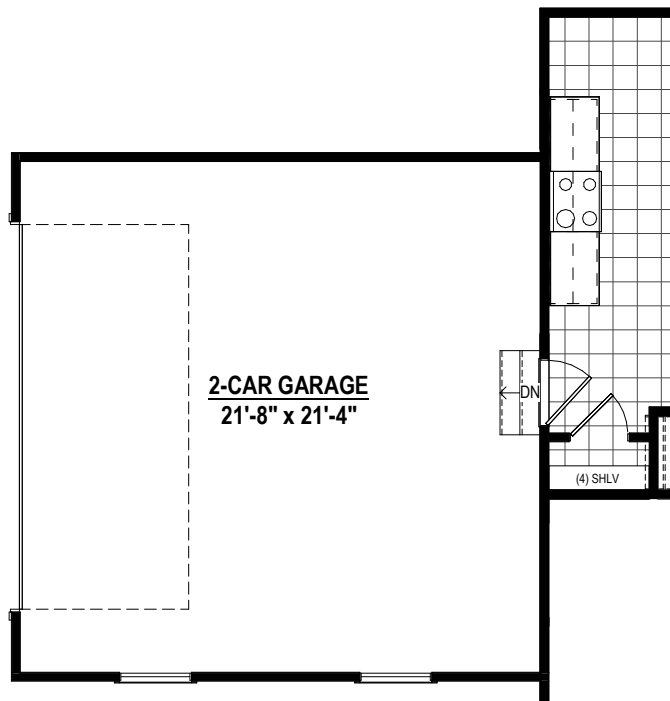
2-CAR SIDE-LOAD GARAGE (484 SF ±) 8'-0" Option #15238 9'-0" Option #15260
