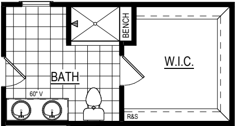
PRIMARY BATH W/ SHOWER BENCH Option #65025
