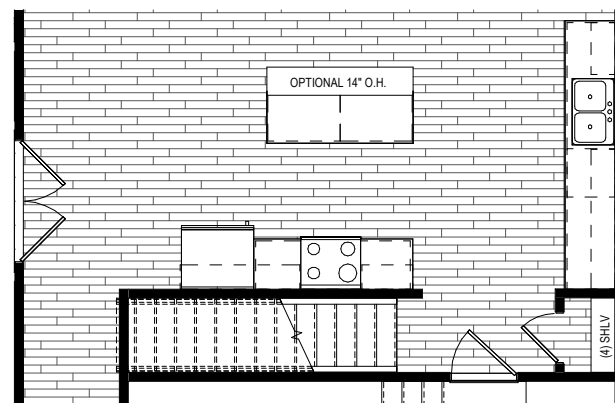
24"X48" KITCHEN ISLAND W/ O.H.
