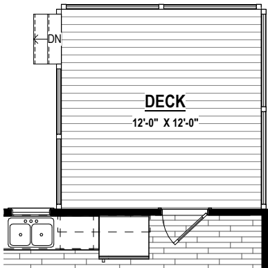
DECK (144 SF ±) Wood Option #15001 Trex Option #15011
