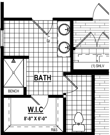
PRIMARY BATH W/ SHOWER BENCH 8'-0" Option #65025 9'-0" Option #65030
