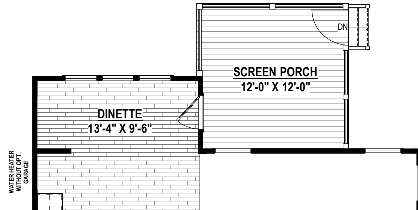
SCREEN PORCH W/ DINETTE (147 SF ± 84 SF ±) 8'-0" Option #15047 Wood Option #15501 9'-0" Option #15046 Trex Option #15511
