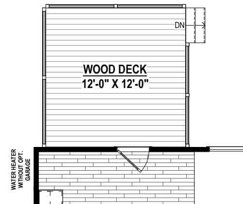
DECK (144 SF ±) Wood Option #15001 Trex Option #15011
