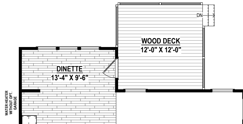
WOOD DECK W/ DINETTE (144 SF ± 84 SF ±) 8'-0" Option #15047 Wood Option #15001 9'-0" Option #15046 Trex Option #15011
