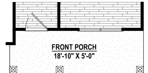
FULL FRONT PORCH (92 SF ±) Option #15240
