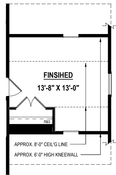
FINISHED ROOM OVER 1-CAR GARAGE (182 S/F ±) Option #15033
