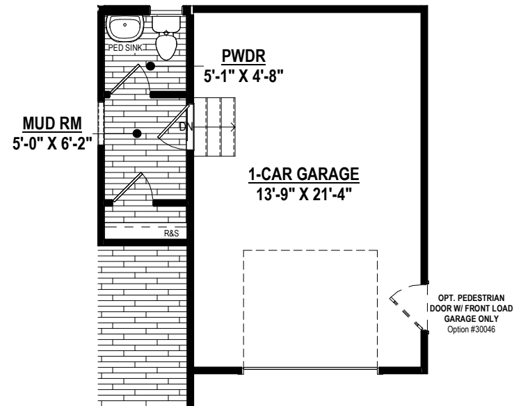
1-CAR FRONT-LOAD GARAGE (308 SF ±) 8'-0" Option #15025 9'-0" Option #15035
