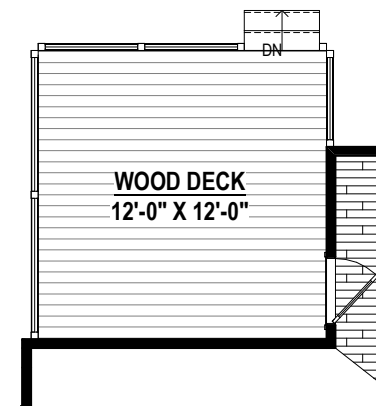
WOOD DECK (144 SF ±) Wood Option #15001 Trex Option #15011
