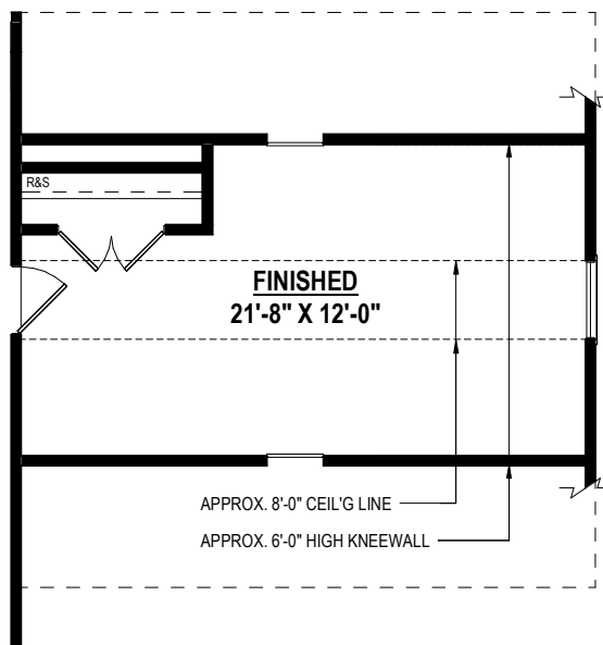
FINISHED ROOM OVER 2-CAR GARAGE (279 SF ±) Option #15034
