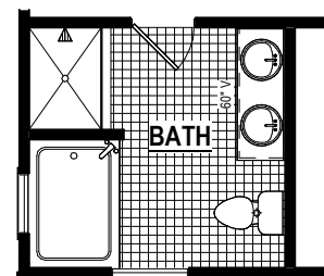
PRIMARY BATH W/ SOAKING TUB Option #41150
