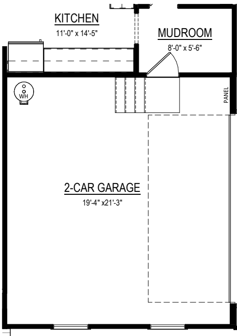
2-CAR SIDE-LOAD GARAGE (423 SF ±) 8'-0" Option #15238 9'-0" Option #15260
