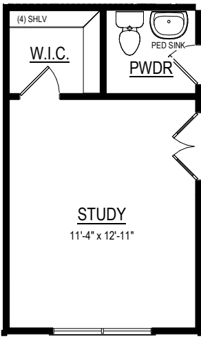
STUDY IN LIEU OF FLEX 8'-0" Option #15116 9'-0" Option #15117
