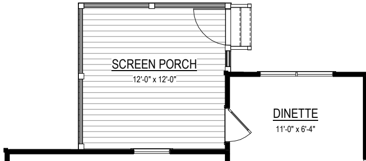
SCREEN PORCH (144 SF ±) Wood Option #15501 Trex Option #15511
