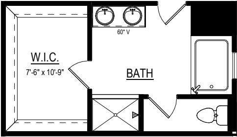
PRIMARY BATH W/ SOAKING TUB Option #41150
