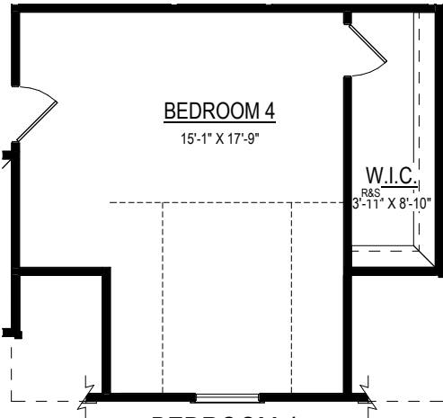
BEDROOM 4 (282 SF ±) Option #15110
