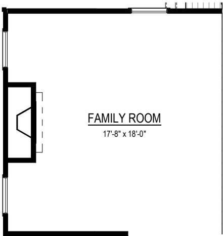
FAMILY ROOM 17'-8" x 18'-0" GAS FIREPLACE AT FAMILY ROOM Option #35005
