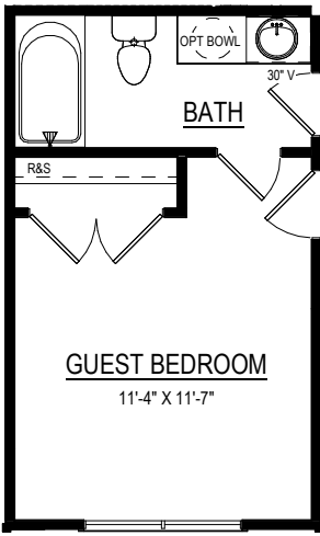
GUEST BEDROOM W/ FULL BATH 8'-0" Option #15097 9'-0" Option #15098
