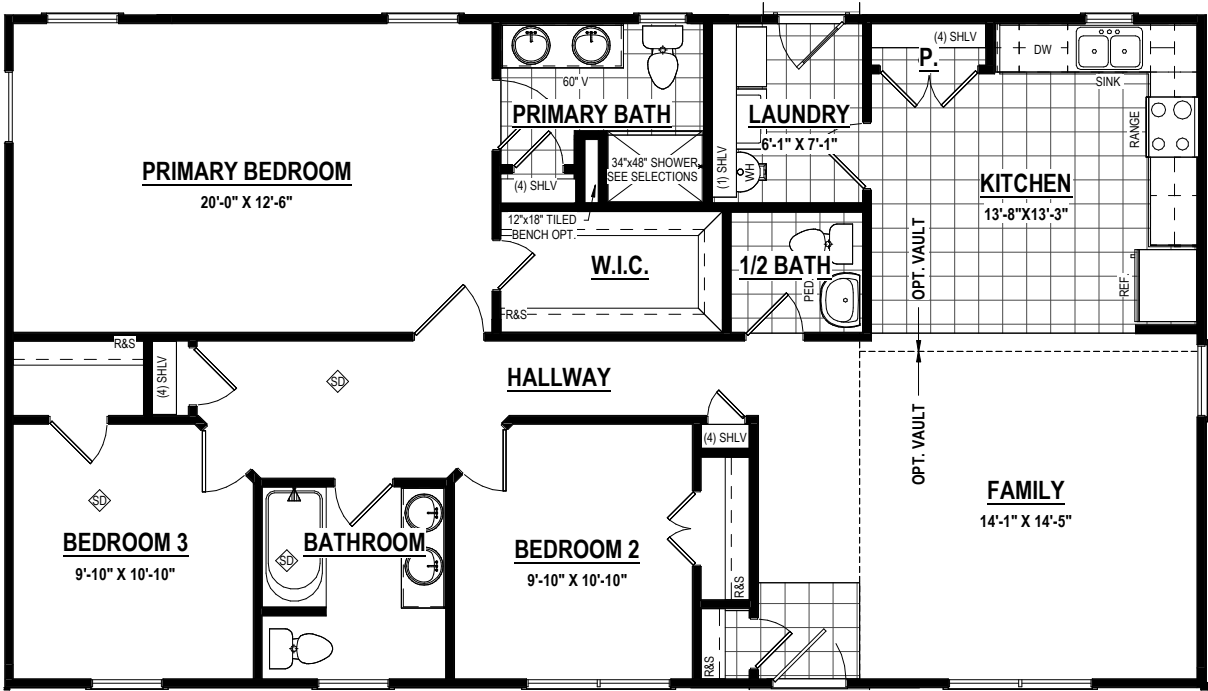
LARGER FLOORPLAN 2 1/2 BATH (248 SF ±) (8' - 0") Option #15150 (9' - 0") Option #15151
