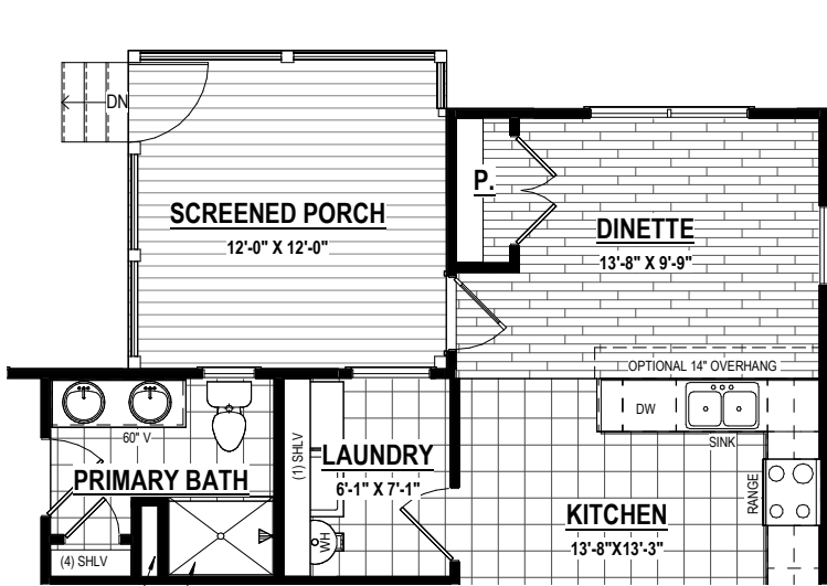
DINETTE W/ SCREENED PORCH (128 SF ±) (Wood) Option #15501 (Trex) Option #15511
