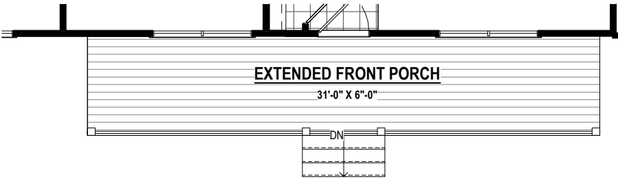
EXTENDED FRONT PORCH (186 SF ±) Option #15248
