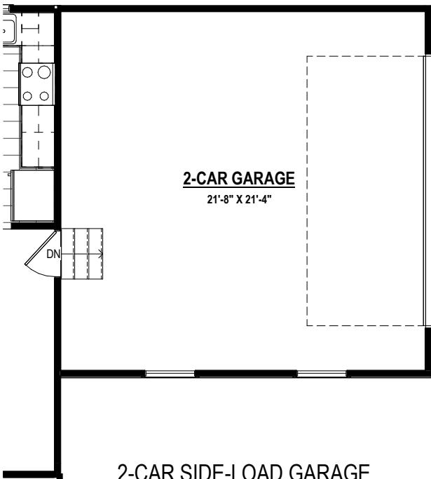
2-CAR SIDE-LOAD GARAGE (484 SF ±)
