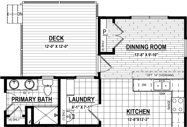
DINETTE W/ DECK (128 SF ±) (Wood) Option #15501 (Trex) Option #15511 (8' - 0") Option #15047 (9' - 0") Option #15046
