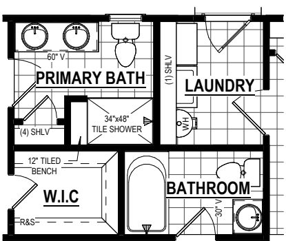
PRIMARY BATHROOM W/ TILE SHOWER W/ BENCH
