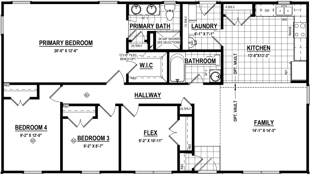
LARGER FLOORPLAN 3 BEDROOM (248 SF ±) (8' - 0") Option #15154 (9' - 0") Option #15155
