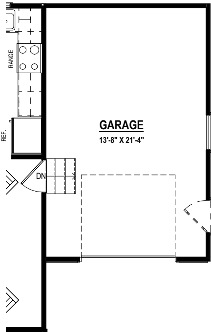
1-CAR FRONT-LOAD GARAGE (292 SF ±)
