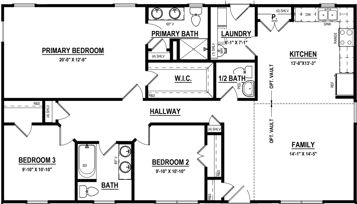
LARGER FLOORPLAN 2 1/2 BATH (248 SF ±)
