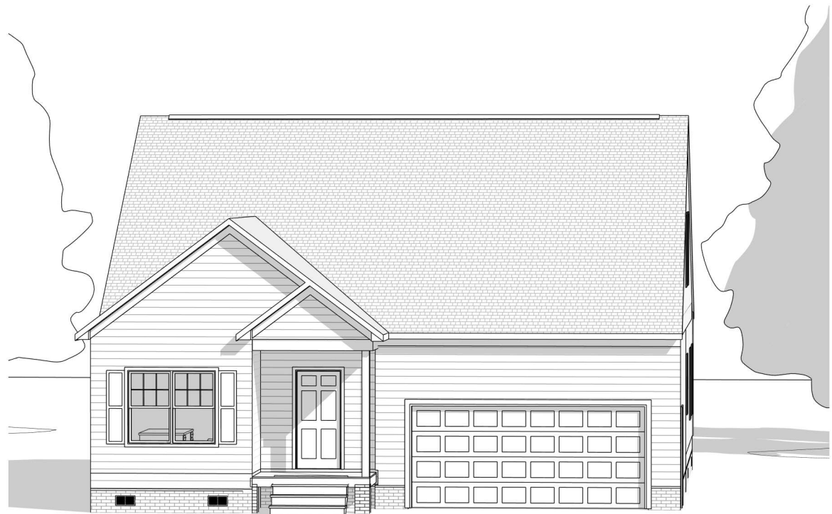
TRADITIONAL ELEVATION
