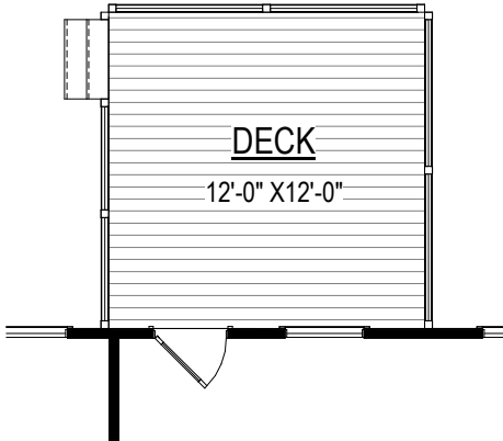
DECK (144 SF ±)
