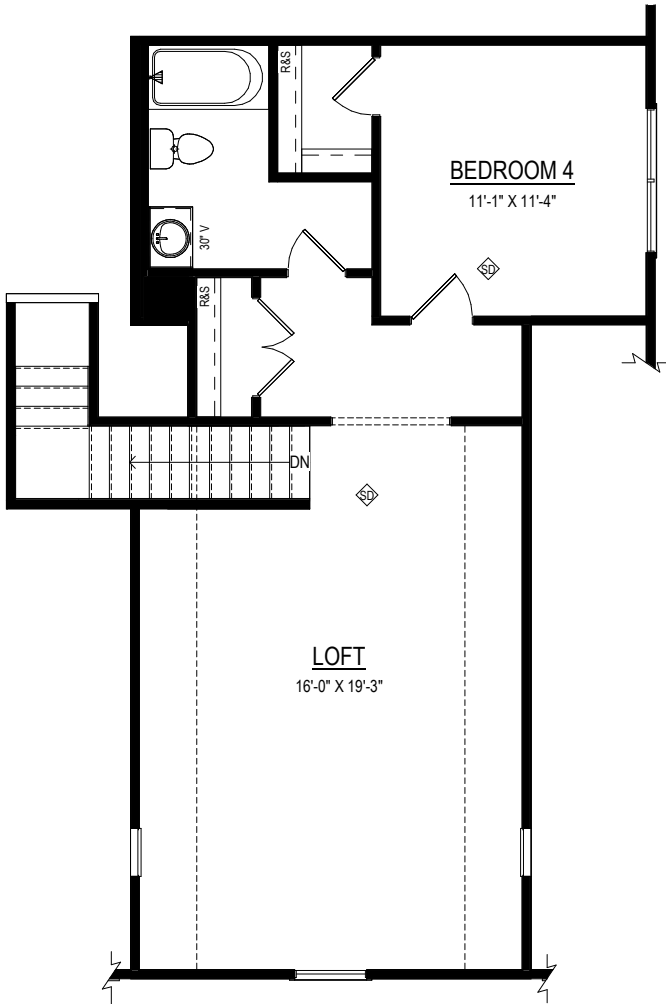
BEDROOM 4 W/ BATH & FINISHED STORAGE (CANNOT HAVE VAULT) (729 SF ±) Option # 15112
