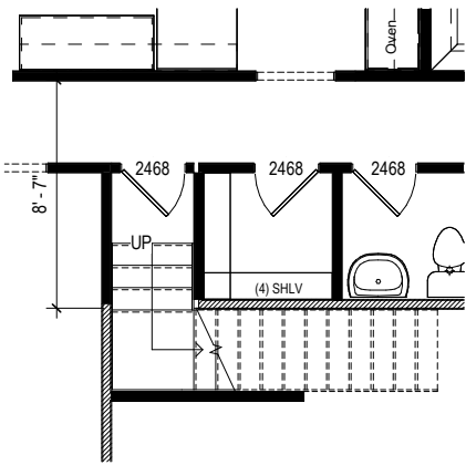
STAIRS TO SECOND FLOOR
