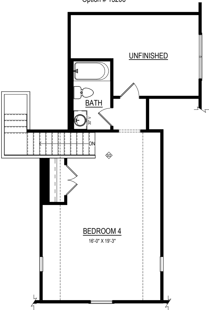
BEDROOM 4 W/ BATH & UNFINISHED STORAGE (488 SF ±) Option # 15111
