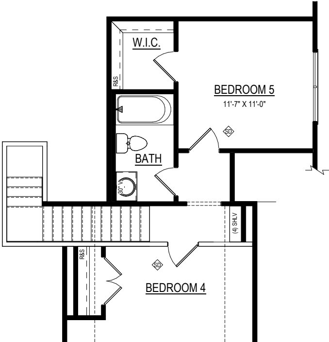
BEDROOM 4 & 5 (662 SF ±) Option # 15206
