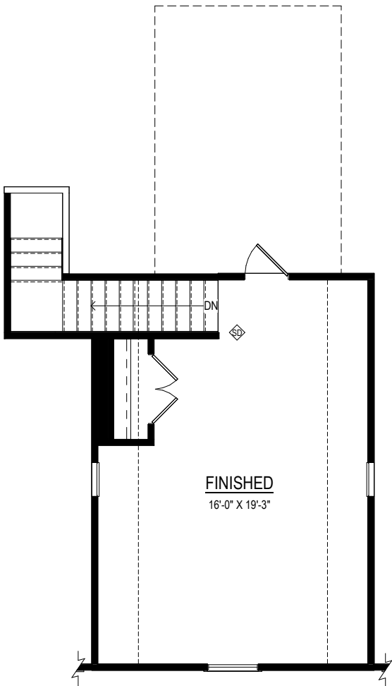
FINISHED W/ UNFINISHED STORAGE (409 SF ±) Option # 15110
