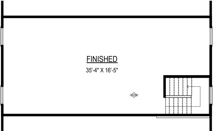
FINISHED THIRD FLOOR Option # 15140 SQ FT FINISHED: 532
