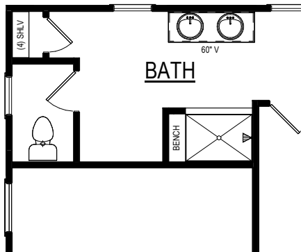
PRIMARY BATH W/ SHOWER BENCH Option #65030
