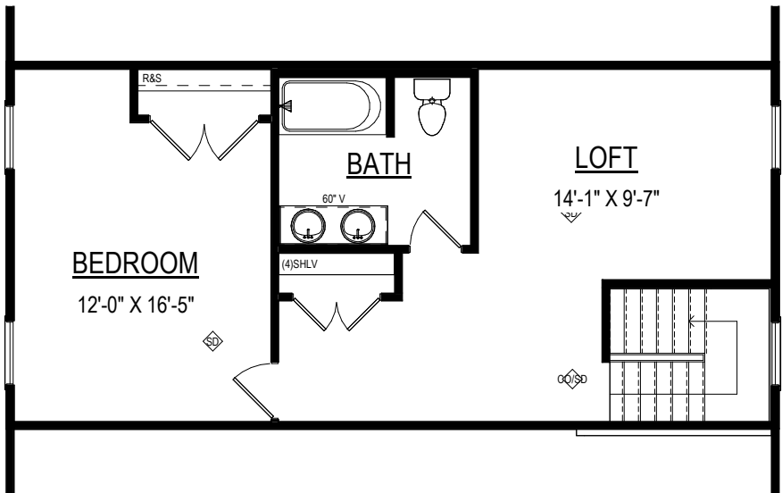
THIRD FLOOR W/ BEDROOM & LOFT Option # 15141 SQ FT FINISHED: 532
