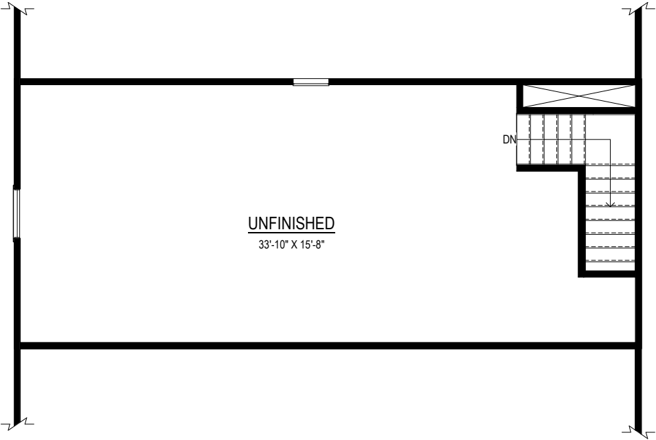
THIRD FLOOR W/ UNFINISHED LOFT
