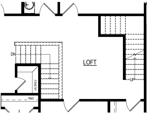
SECOND TO THIRD FLOOR STAIRS - FINISHED
