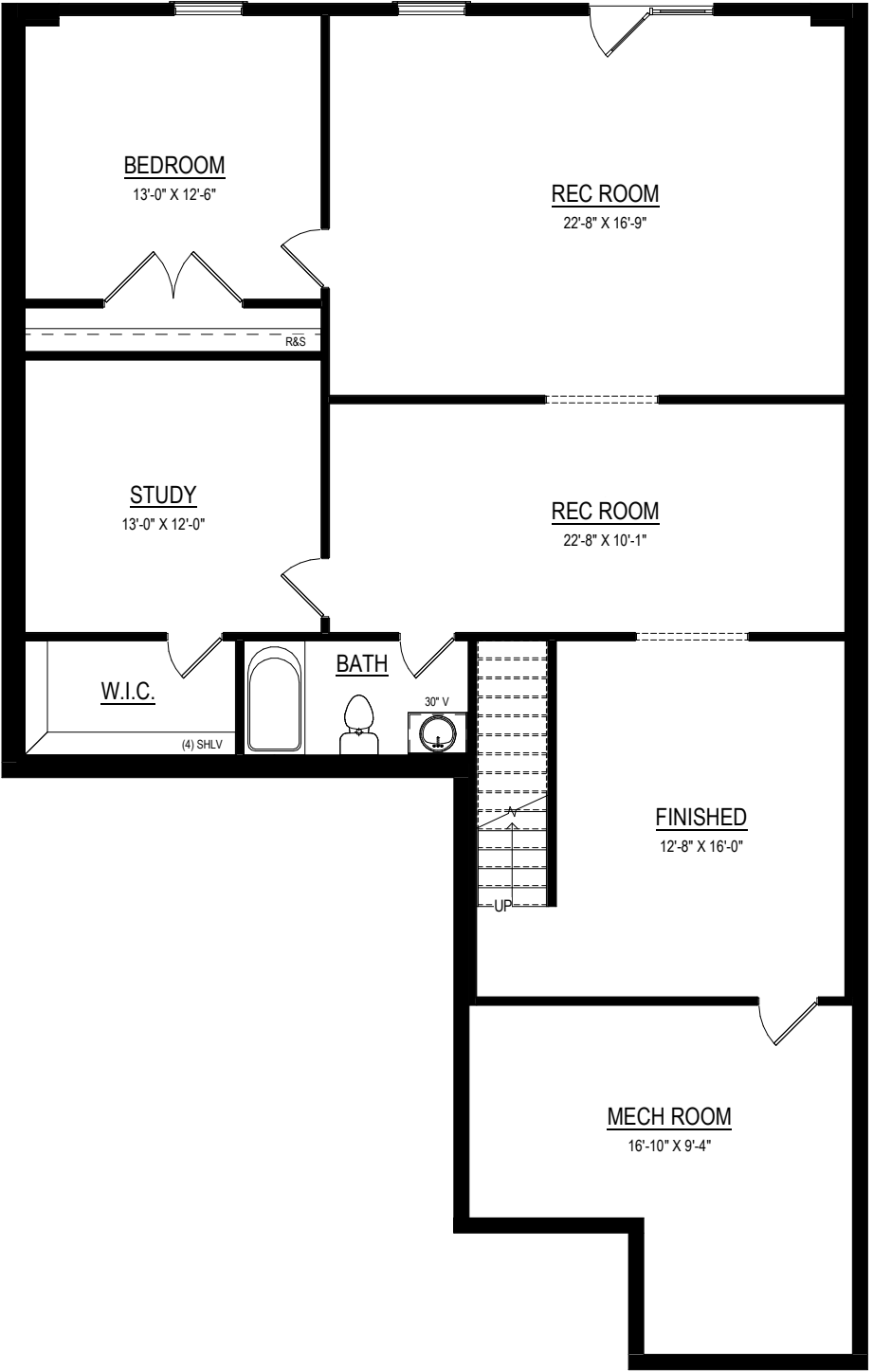
FINISHED BASEMENT - REC ROOM, BEDROOM, STUDY & FULL BATH
