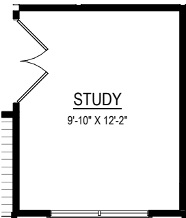
STUDY 9'-10" X 12'-2" STUDY IN LIEU OF FLEX 8' Option # 15116 9' Option # 15117
